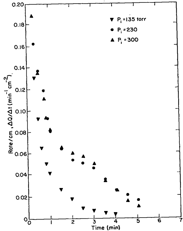
Fig. 3. Rate vs time, 135^{\circ}\text{C} .
