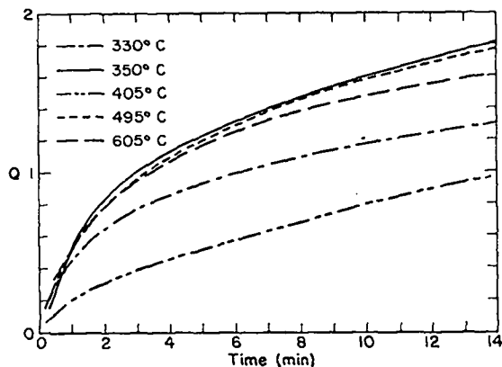
Fig. 7. Q vs time, 330 to 600°C.
