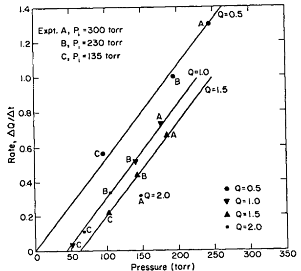
Fig. 4. Rate vs P_D at 135^{\circ}\text{C} and constant Q values.
